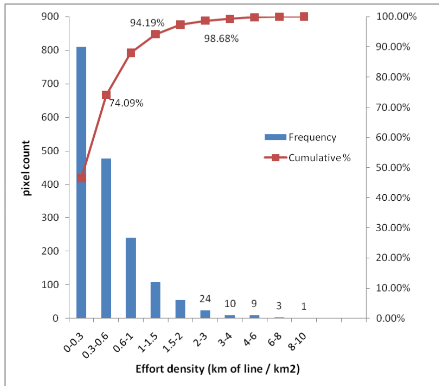
Figure 22 (after Sharp 2010): Spatial concentration of all historical New Zealand fishing effort in the Ross Sea. The histogram sorts 1737 non-zero-effort pixels (0.05° latitude x 0.177° longitude) as a function of cumulative effort density (in km of line per km²). Note that the horizontal scale is not linear and that an additional 115 296 pixels in the Ross Sea with zero New Zealand effort (98.4% of the total) are not shown.
