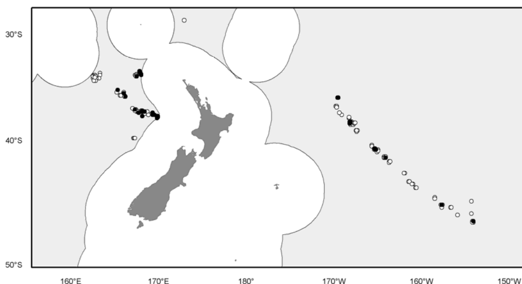
Figure 2. Observed tows (2003-2007) from New Zealand vessels within the SPRFMO area with VME score of three or greater based on the 50th percentile thresholds from 1998-2002 (black circles), or tows with score less than 3 (white circles), (N=1010).
